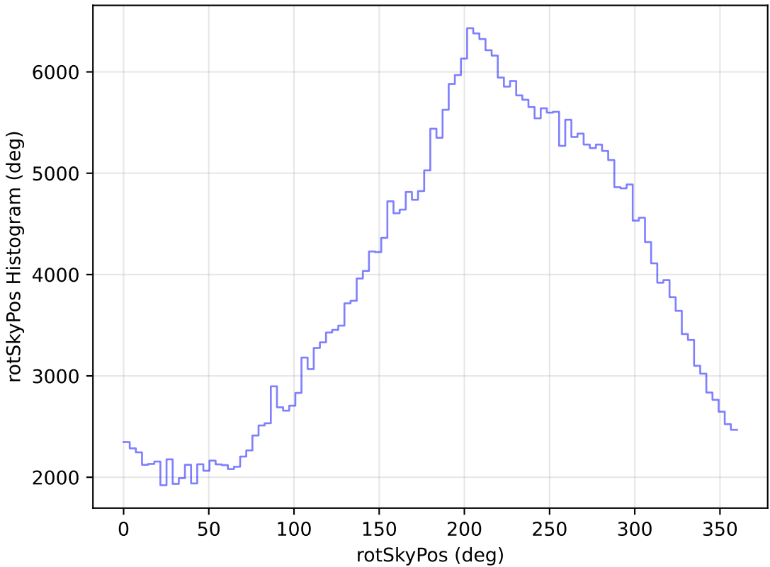
ddf_loaded_fl8_v3.4_10yrs All sky y band: rotSkyPos Histogram
