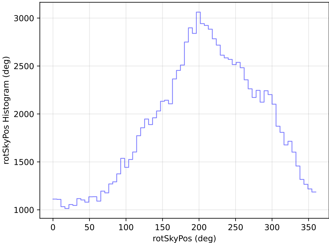
ddf_loaded_fl8_v3.4_10yrs All sky u band: rotSkyPos Histogram
