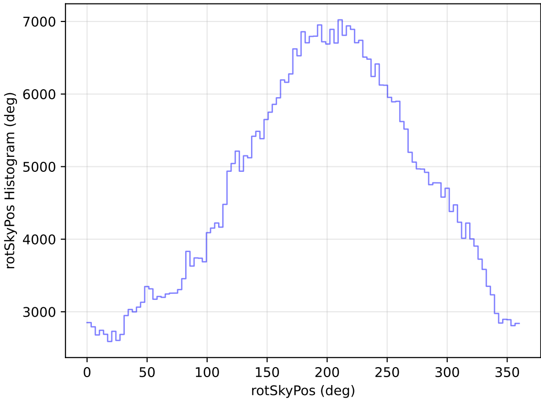
ddf_loaded_fl8_v3.4_10yrs All sky r band: rotSkyPos Histogram
