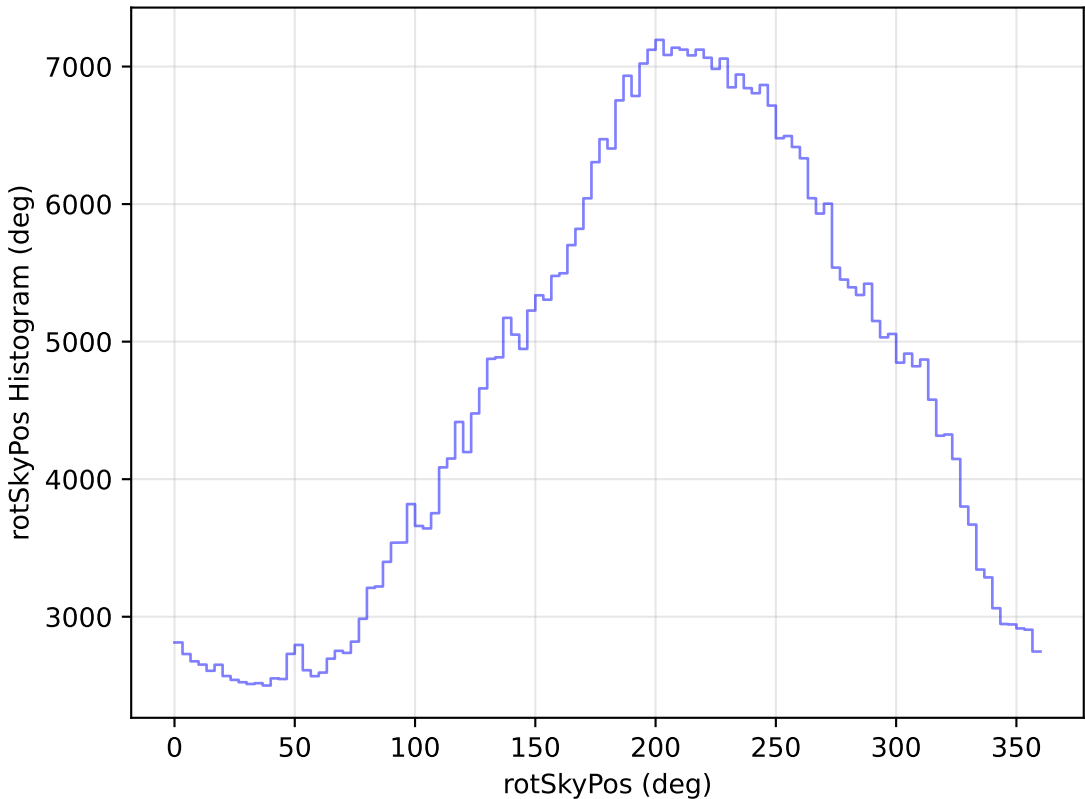
ddf_loaded_fl8_v3.4_10yrs All sky i band: rotSkyPos Histogram
