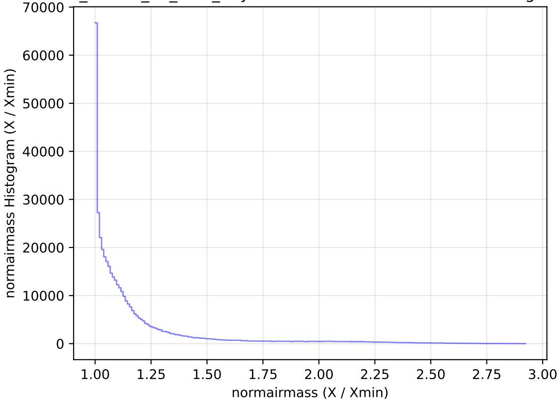
ddf_loaded_fl8_v3.4_10yrs WFD z band: normairmass Histogram
