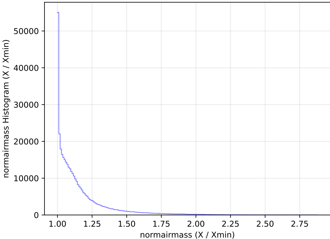
ddf_loaded_fl8_v3.4_10yrs WFD y band: normairmass Histogram
