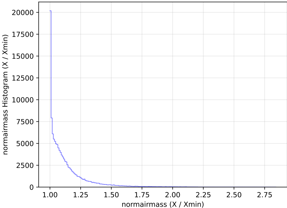
ddf_loaded_fl8_v3.4_10yrs WFD u band: normairmass Histogram
