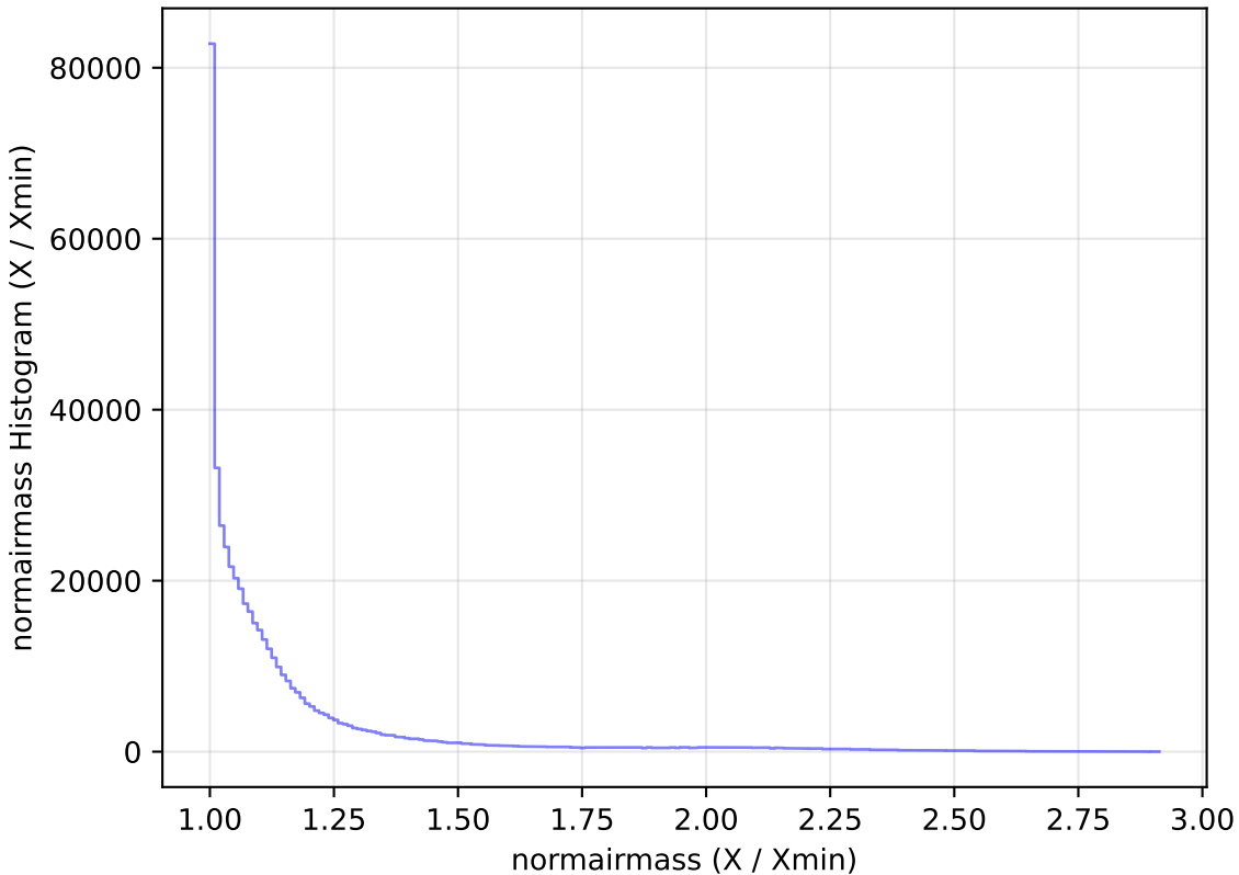
ddf_loaded_fl8_v3.4_10yrs WFD i band: normairmass Histogram
