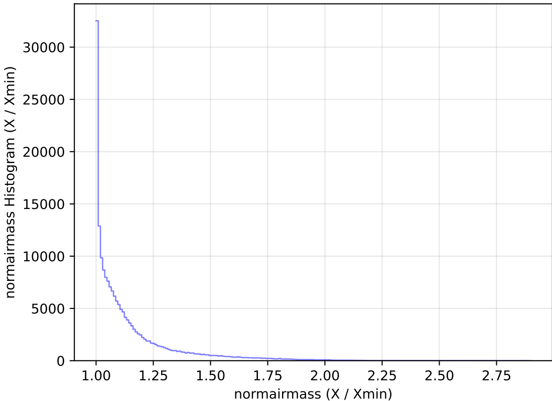
ddf_loaded_fl8_v3.4_10yrs WFD g band: normairmass Histogram
