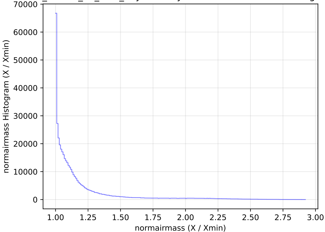
ddf_loaded_fl8_v3.4_10yrs All sky z band: normairmass Histogram
