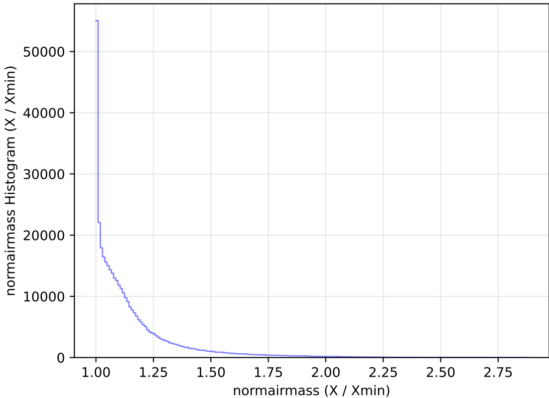
ddf_loaded_fl8_v3.4_10yrs All sky y band: normairmass Histogram
