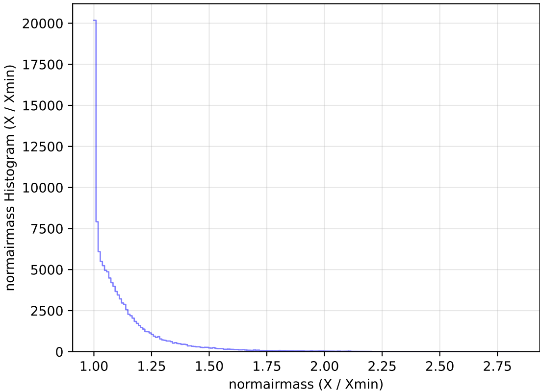
ddf_loaded_fl8_v3.4_10yrs All sky u band: normairmass Histogram
