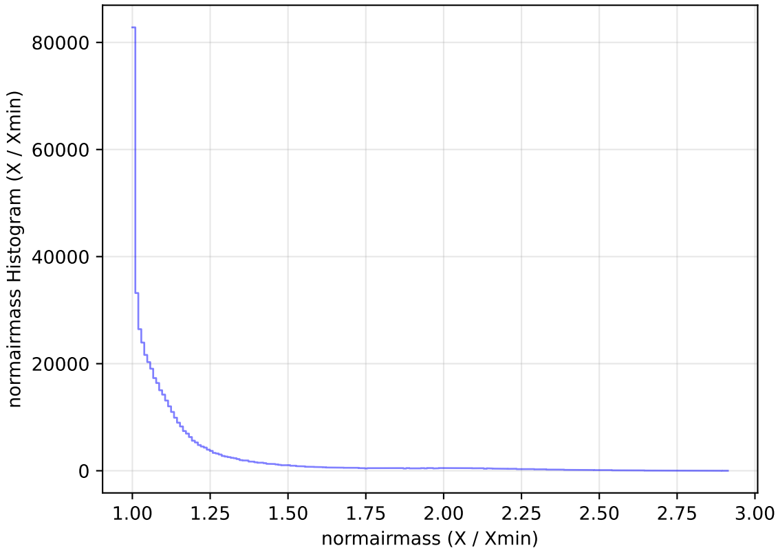
ddf_loaded_fl8_v3.4_10yrs All sky i band: normairmass Histogram
