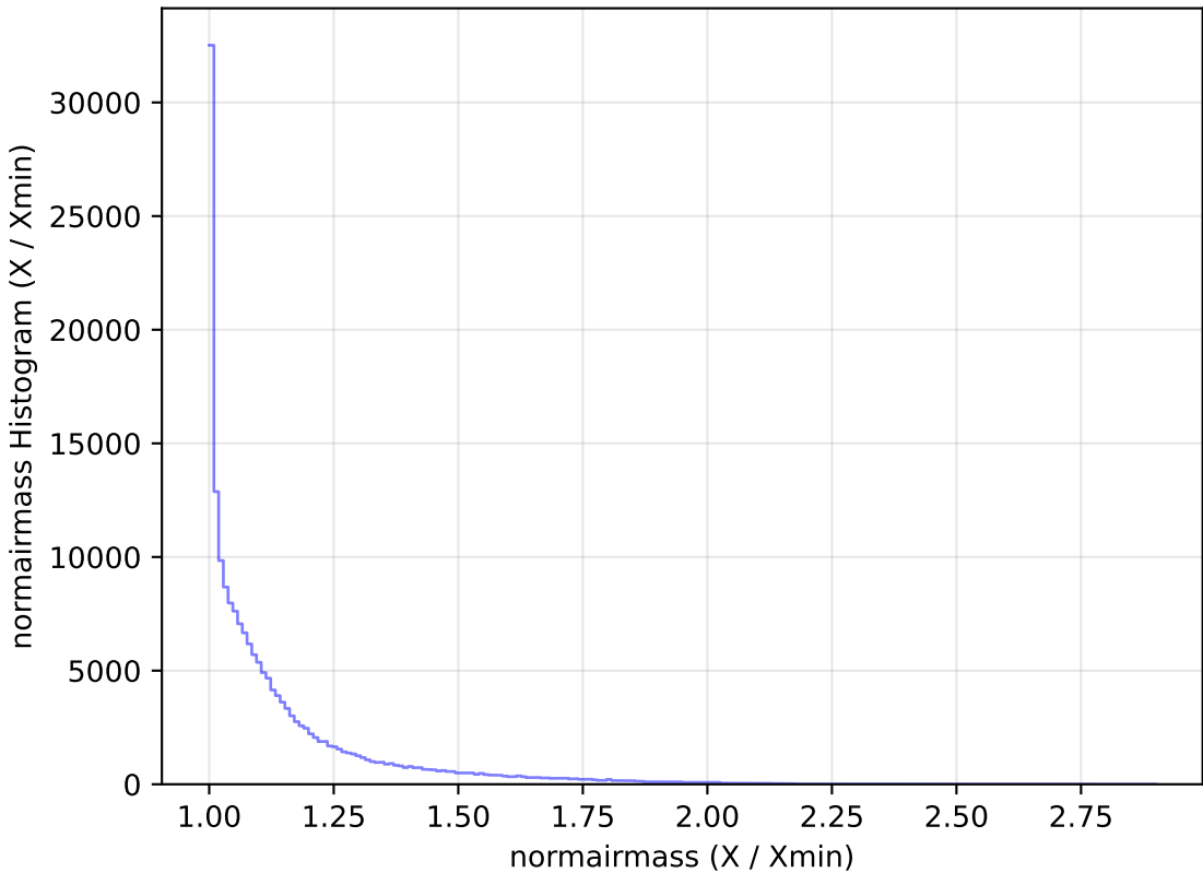
ddf_loaded_fl8_v3.4_10yrs All sky g band: normairmass Histogram
