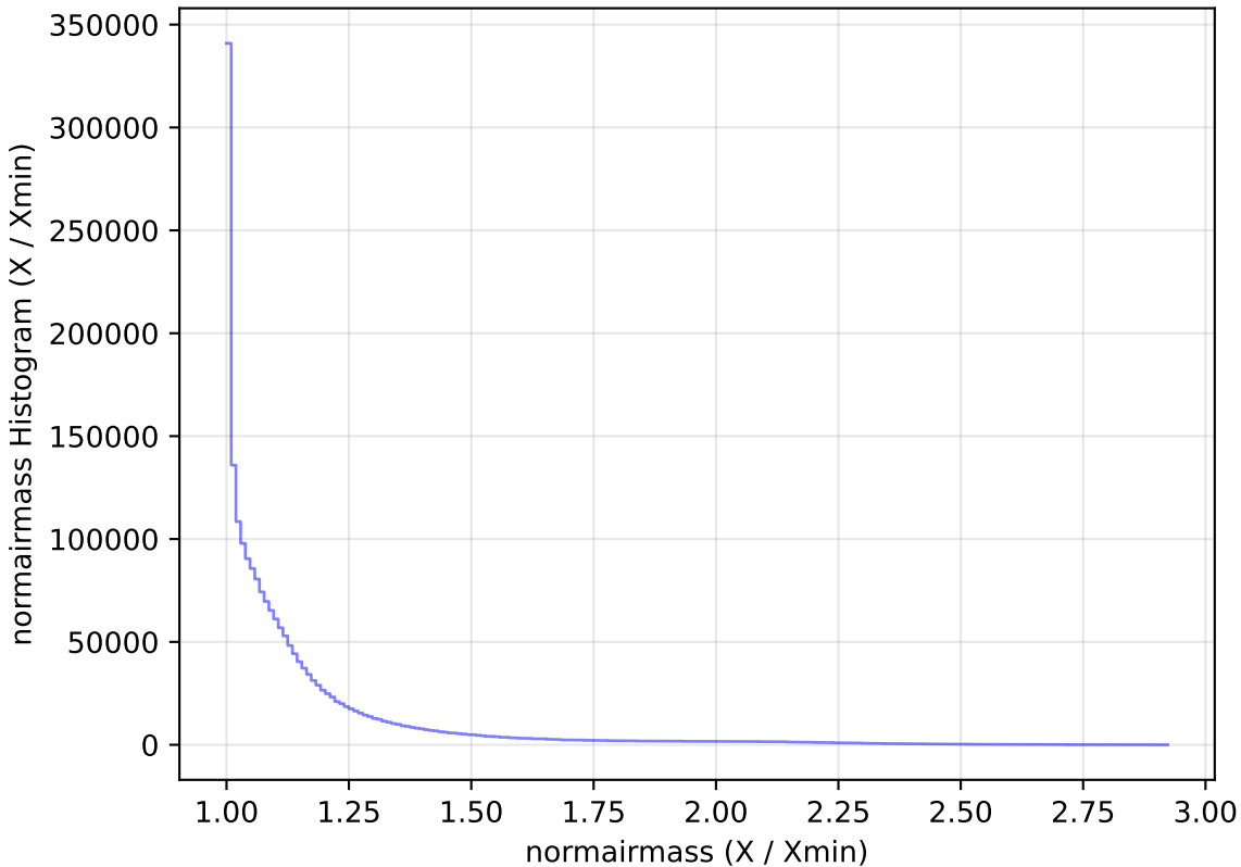
ddf_loaded_fl8_v3.4_10yrs All sky all bands: normairmass Histogram
