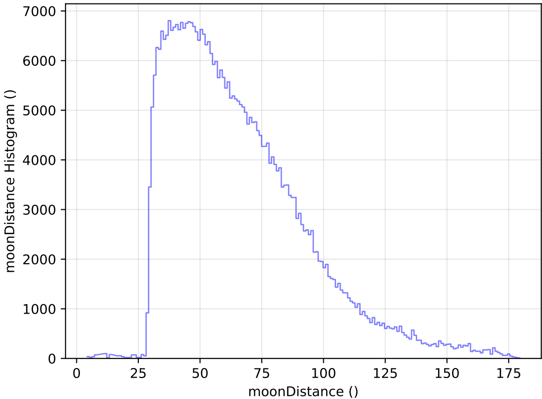
ddf_loaded_fl8_v3.4_10yrs WFD y band: moonDistance Histogram
