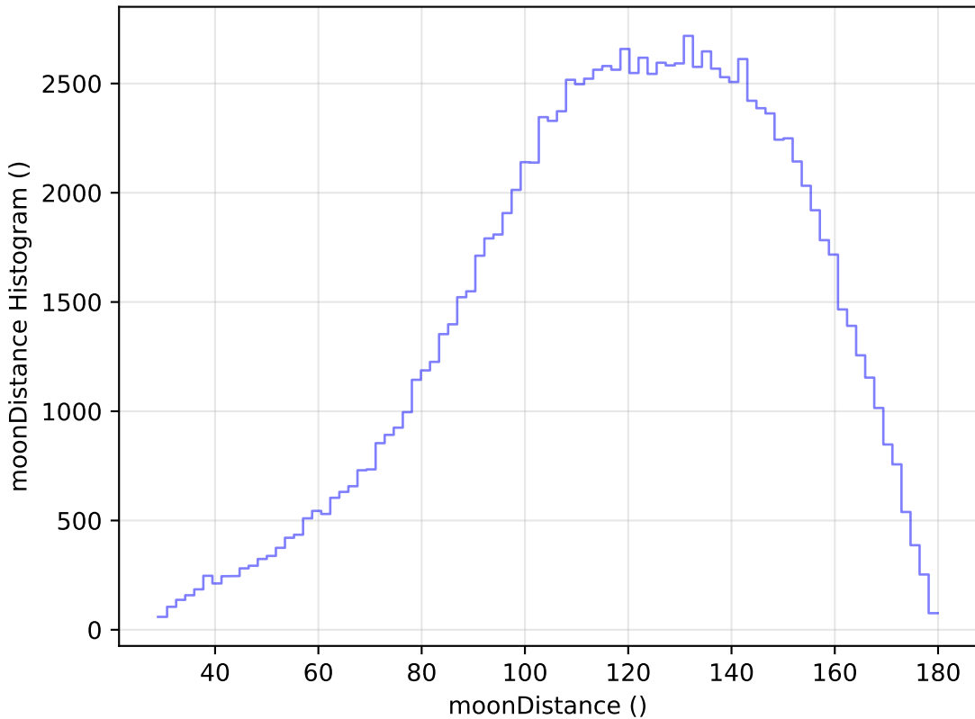
ddf_loaded_fl8_v3.4_10yrs WFD u band: moonDistance Histogram
