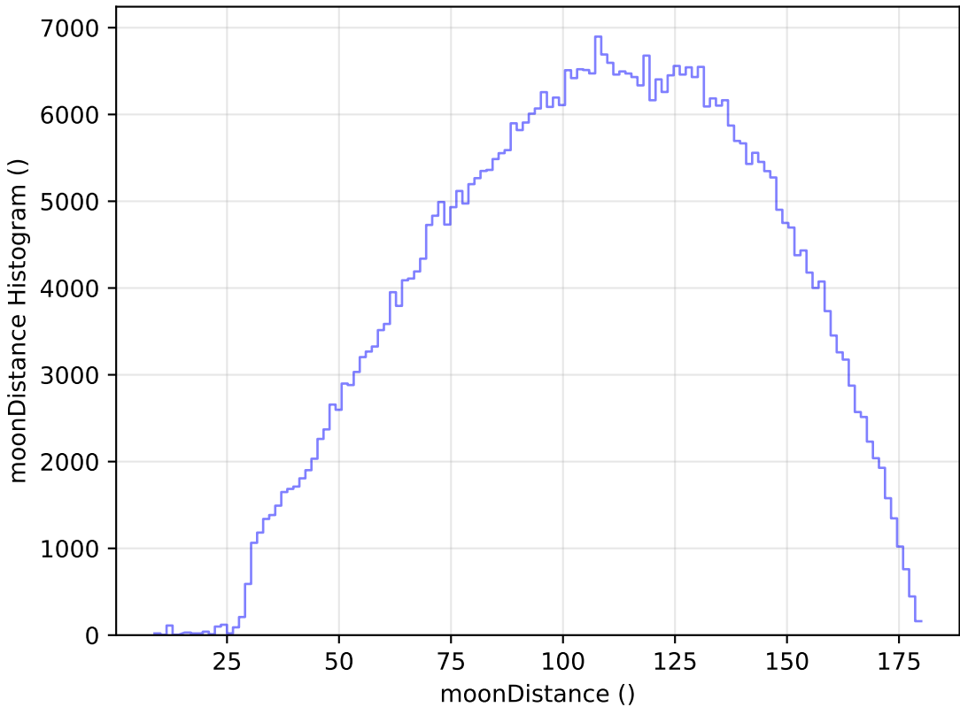
ddf_loaded_fl8_v3.4_10yrs WFD r band: moonDistance Histogram
