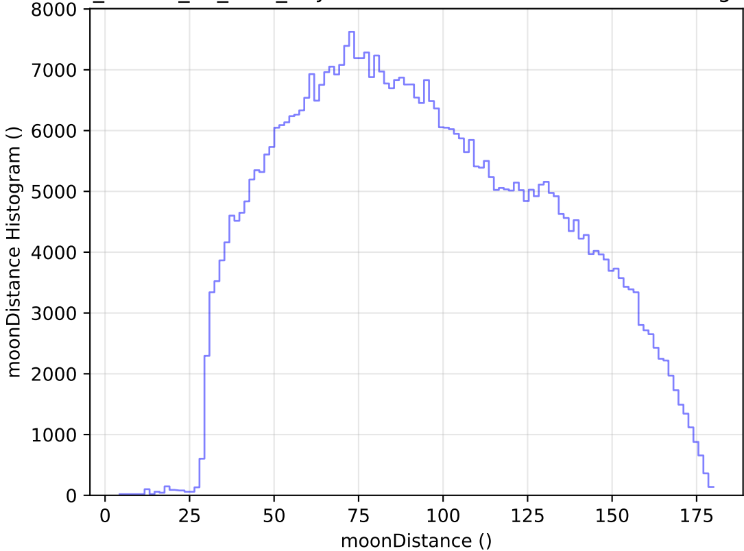
ddf_loaded_fl8_v3.4_10yrs WFD i band: moonDistance Histogram
