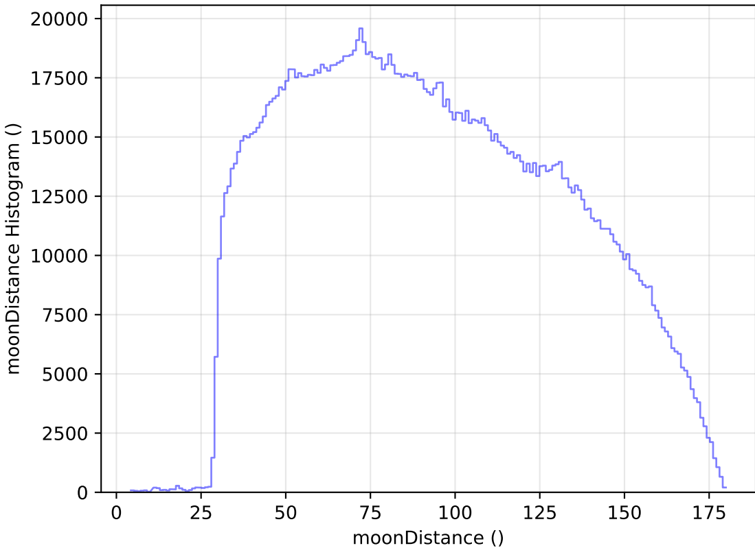
ddf_loaded_fl8_v3.4_10yrs WFD all bands: moonDistance Histogram
