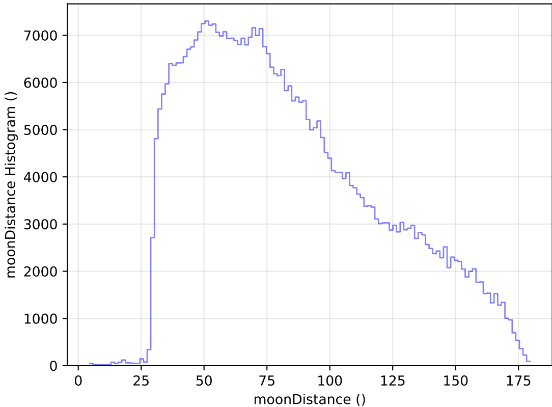
ddf_loaded_fl8_v3.4_10yrs All sky z band: moonDistance Histogram
