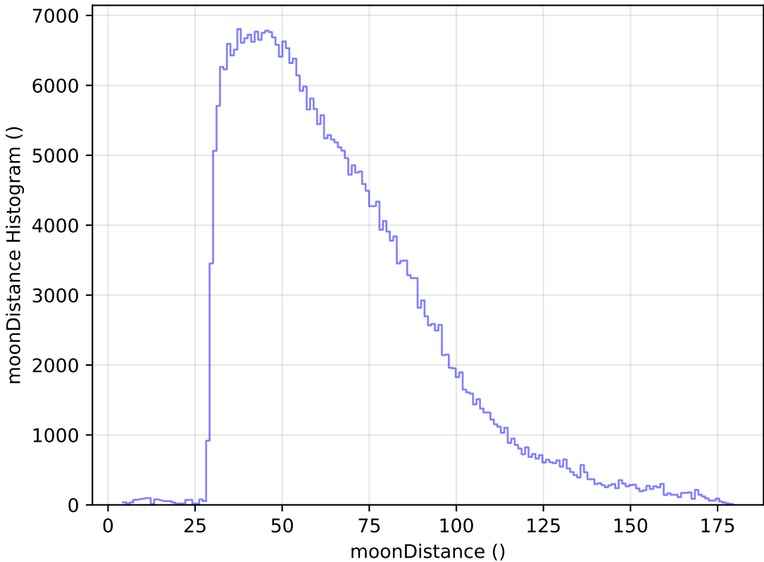
ddf_loaded_fl8_v3.4_10yrs All sky y band: moonDistance Histogram
