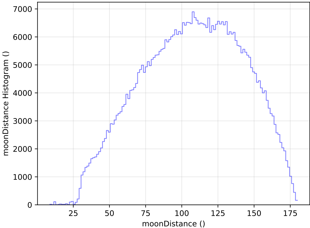
ddf_loaded_fl8_v3.4_10yrs All sky r band: moonDistance Histogram
