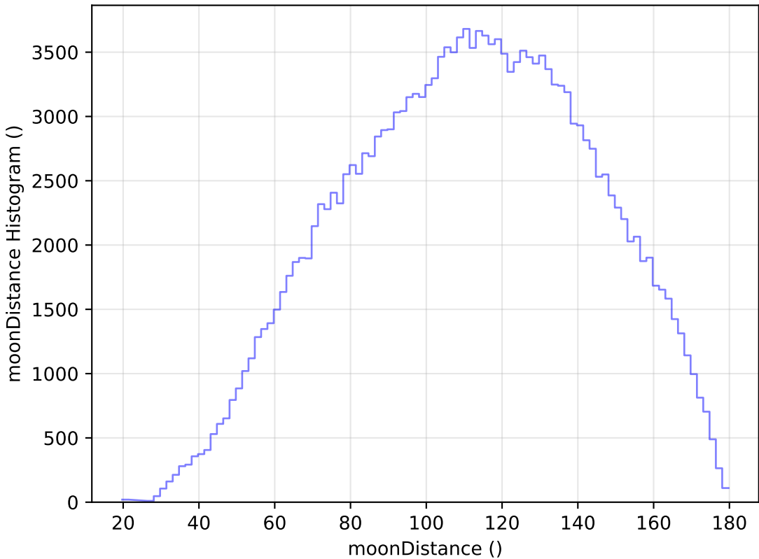
ddf_loaded_fl8_v3.4_10yrs All sky g band: moonDistance Histogram
