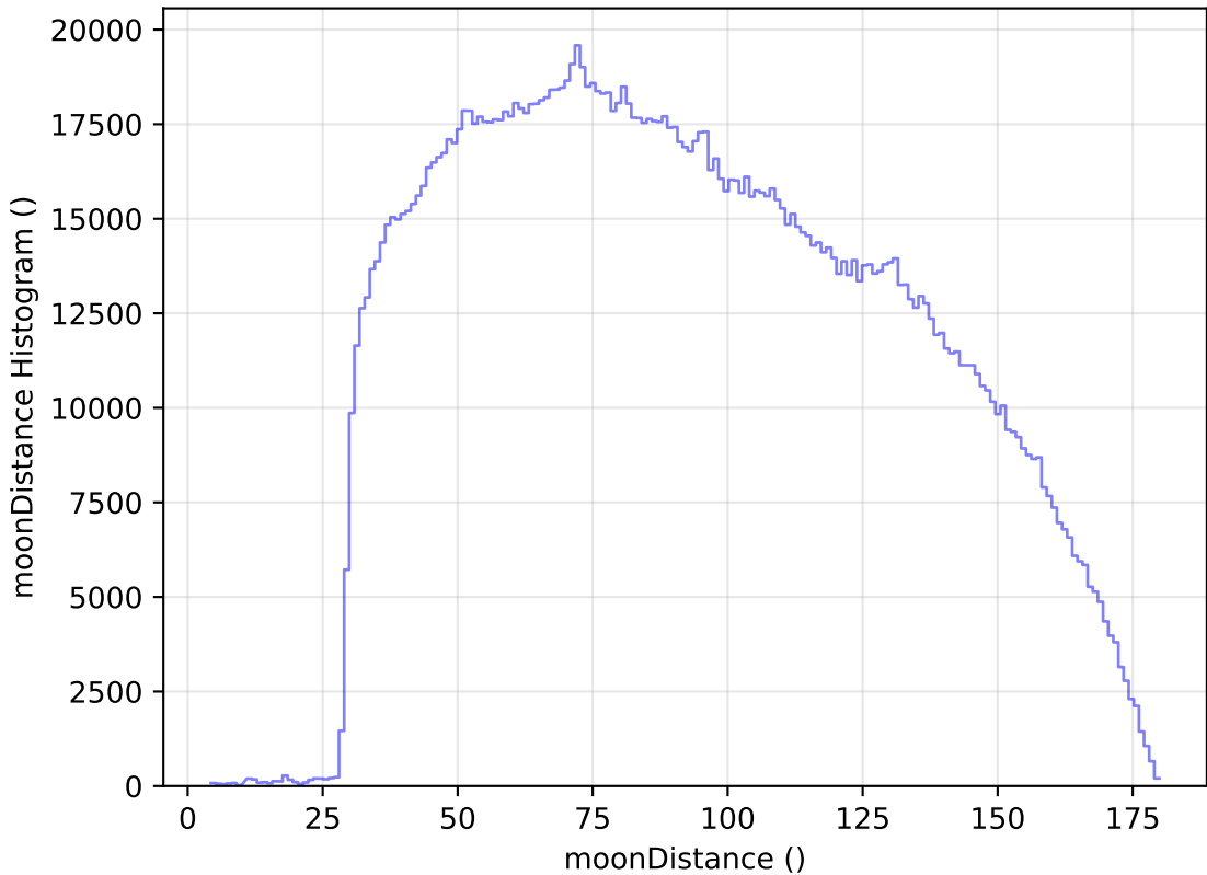
ddf_loaded_fl8_v3.4_10yrs All sky all bands: moonDistance Histogram
