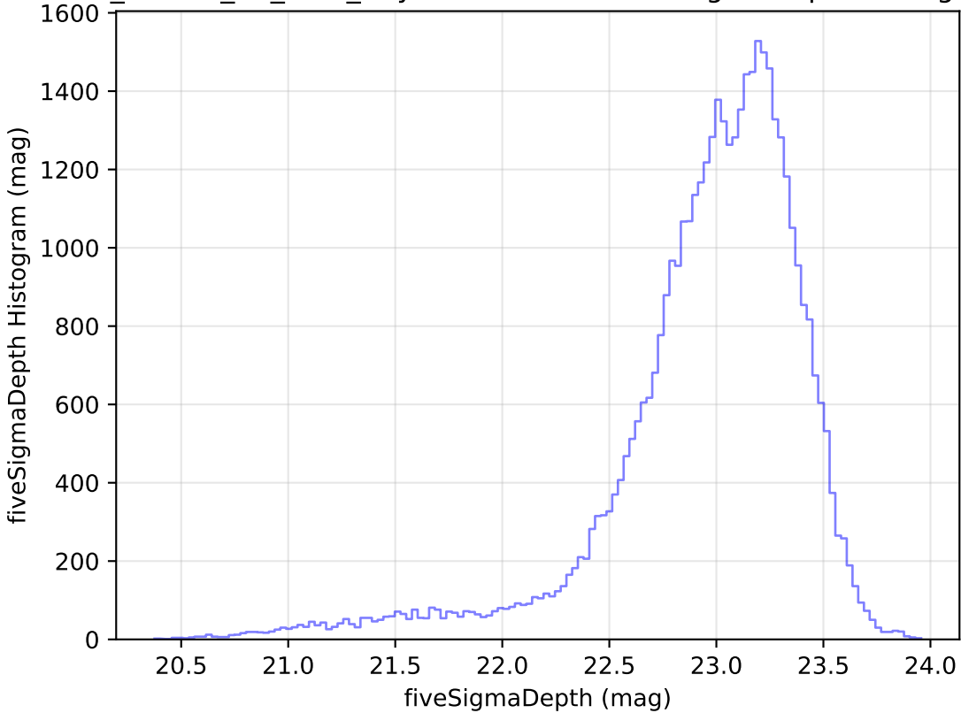
ddf_loaded_fl8_v3.4_10yrs Yr 1 z band: fiveSigmaDepth Histogram
