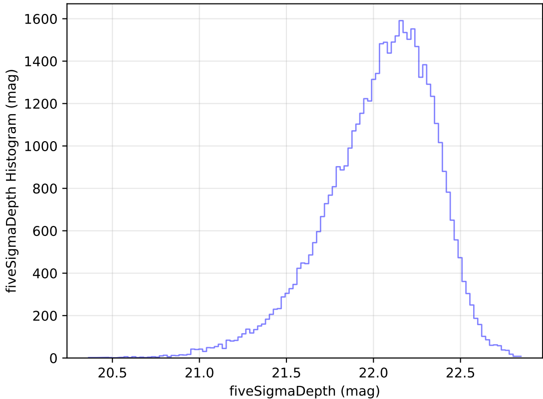
ddf_loaded_fl8_v3.4_10yrs Yr 1 y band: fiveSigmaDepth Histogram
