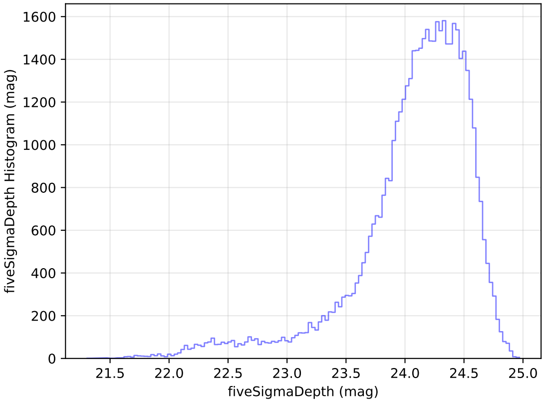
ddf_loaded_fl8_v3.4_10yrs Yr 1 r band: fiveSigmaDepth Histogram
