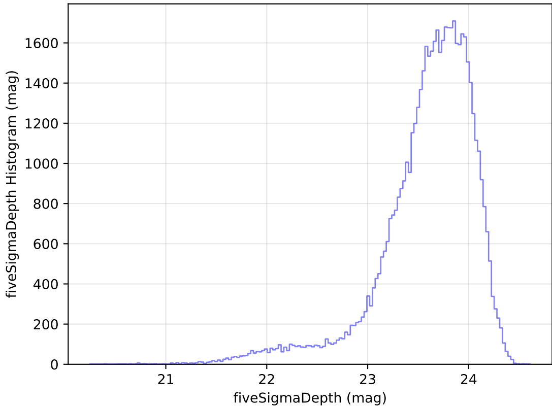
ddf_loaded_fl8_v3.4_10yrs Yr 1 i band: fiveSigmaDepth Histogram
