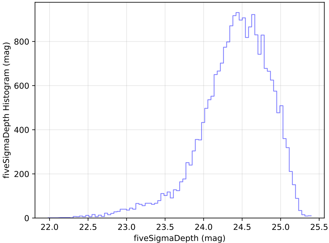
ddf_loaded_fl8_v3.4_10yrs Yr 1 g band: fiveSigmaDepth Histogram
