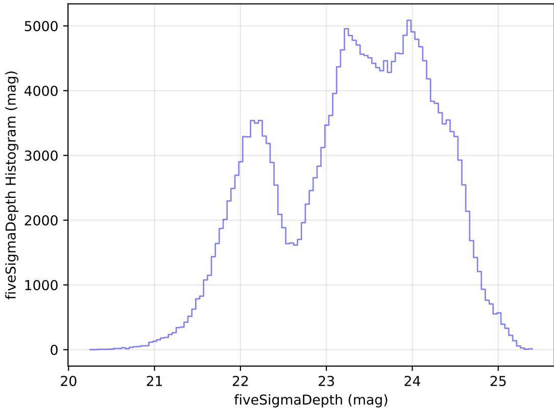
ddf_loaded_fl8_v3.4_10yrs Yr 1 all bands: fiveSigmaDepth Histogram
