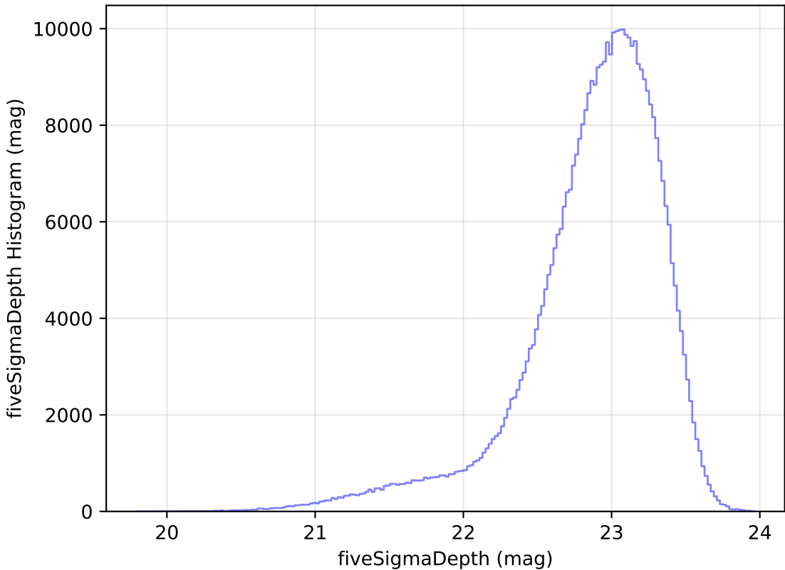
ddf_loaded_fl8_v3.4_10yrs WFD z band: fiveSigmaDepth Histogram
