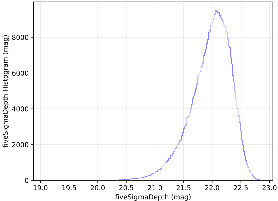
ddf_loaded_fl8_v3.4_10yrs WFD y band: fiveSigmaDepth Histogram
