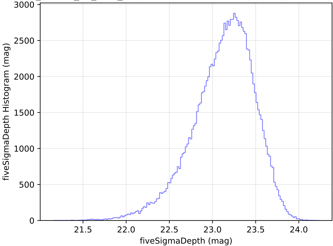
ddf_loaded_fl8_v3.4_10yrs WFD u band: fiveSigmaDepth Histogram
