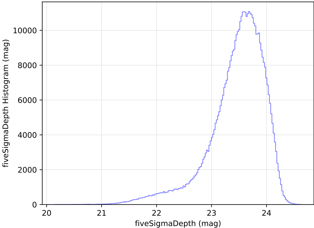
ddf_loaded_fl8_v3.4_10yrs WFD i band: fiveSigmaDepth Histogram
