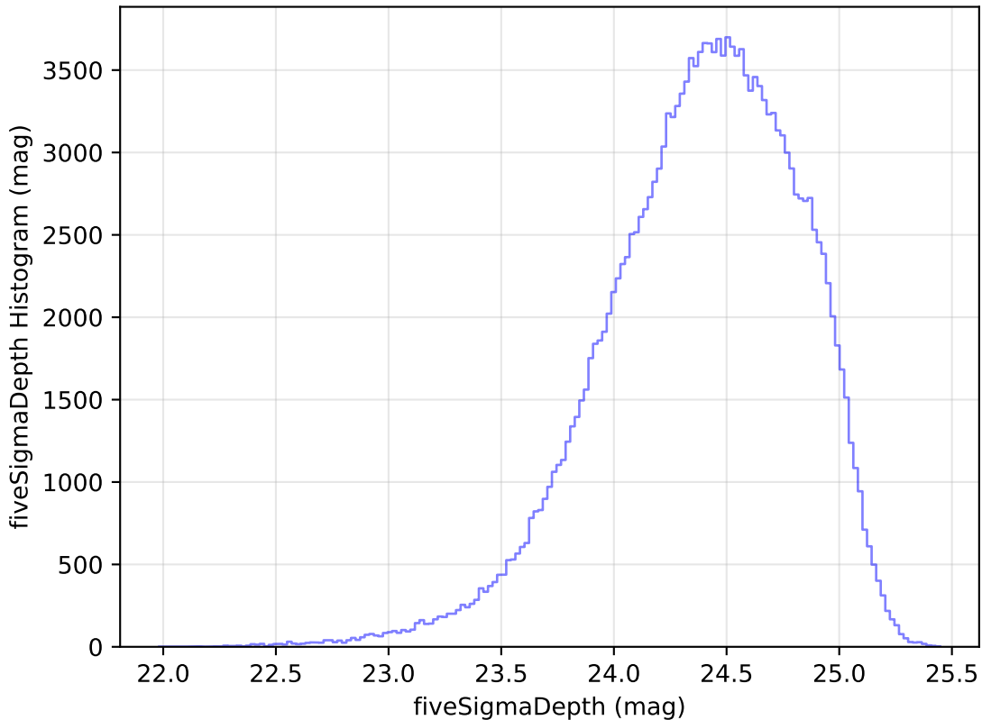
ddf_loaded_fl8_v3.4_10yrs WFD g band: fiveSigmaDepth Histogram
