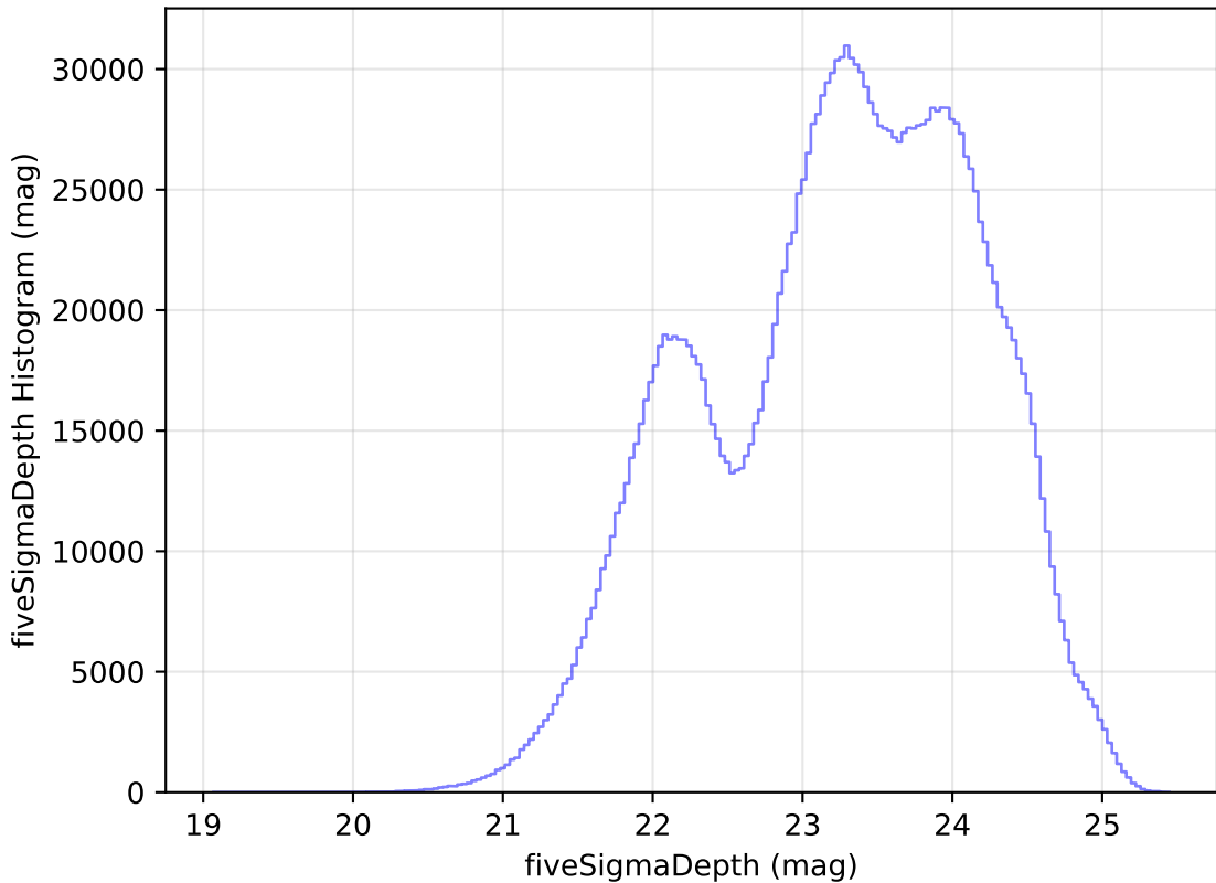
ddf_loaded_fl8_v3.4_10yrs WFD all bands: fiveSigmaDepth Histogram
