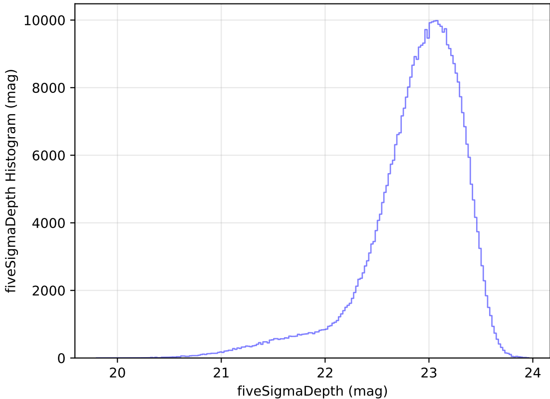
ddf_loaded_fl8_v3.4_10yrs All sky z band: fiveSigmaDepth Histogram
