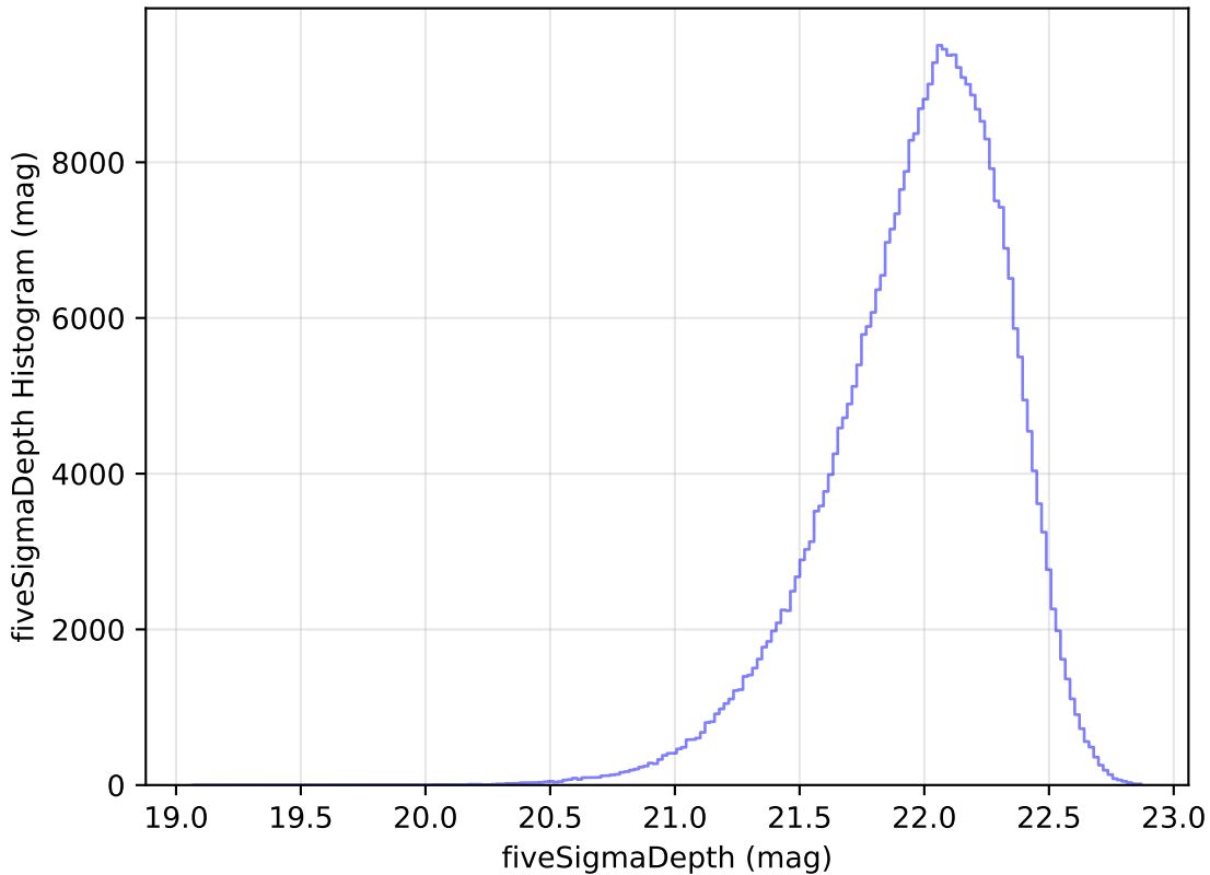
ddf_loaded_fl8_v3.4_10yrs All sky y band: fiveSigmaDepth Histogram
