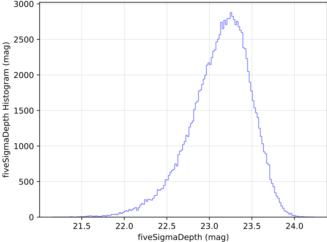
ddf_loaded_fl8_v3.4_10yrs All sky u band: fiveSigmaDepth Histogram
