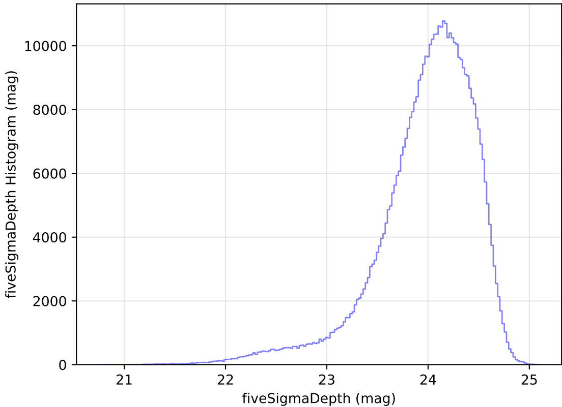
ddf_loaded_fl8_v3.4_10yrs All sky r band: fiveSigmaDepth Histogram
