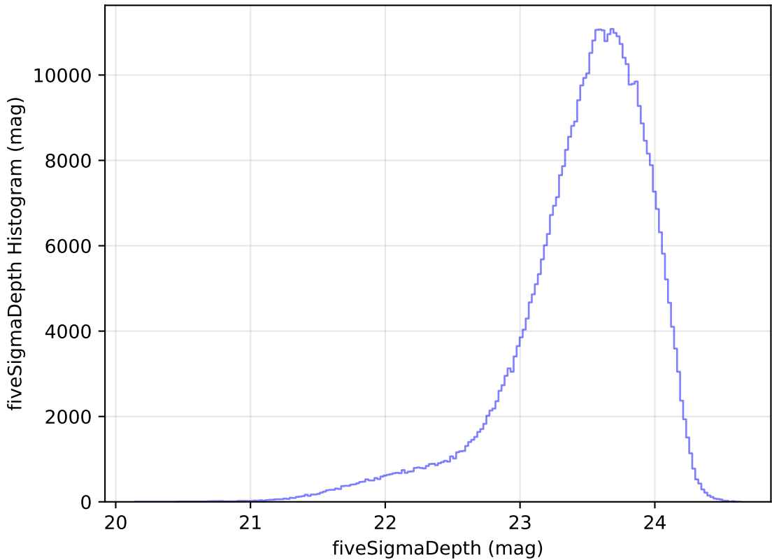
ddf_loaded_fl8_v3.4_10yrs All sky i band: fiveSigmaDepth Histogram
