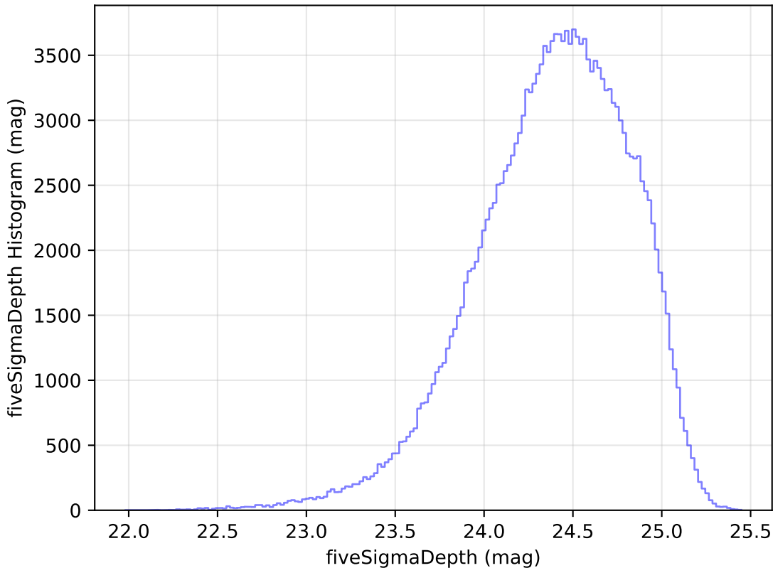
ddf_loaded_fl8_v3.4_10yrs All sky g band: fiveSigmaDepth Histogram
