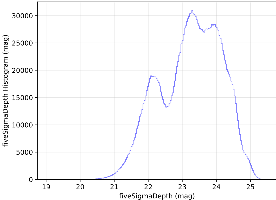
ddf_loaded_fl8_v3.4_10yrs All sky all bands: fiveSigmaDepth Histogram
