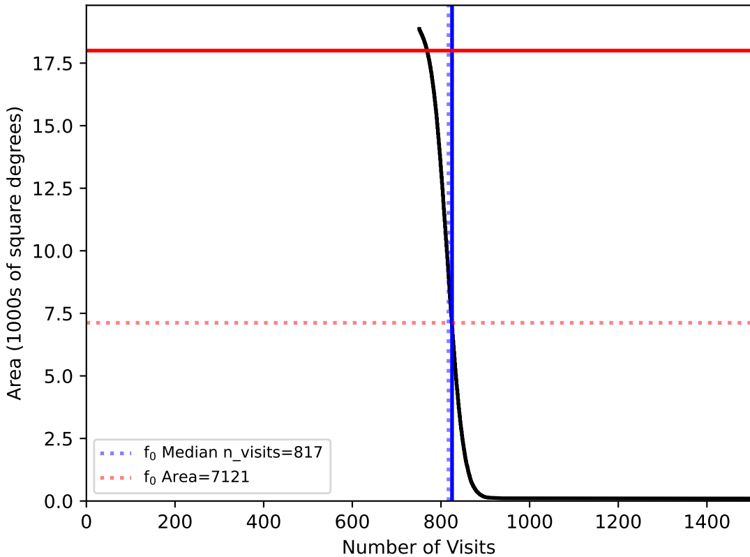
ddf_loaded_fl8_v3.4_10yrs WFD: fO
