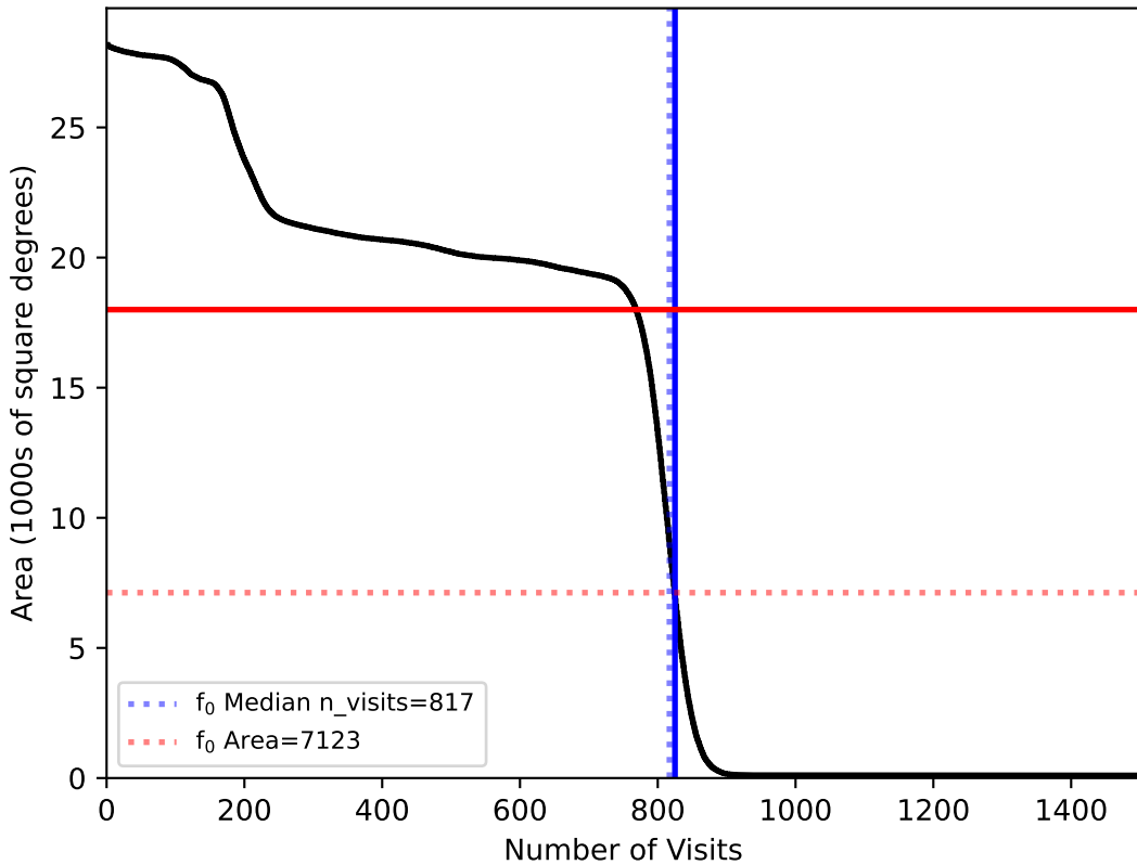
ddf_loaded_fl8_v3.4_10yrs All sky: f0
