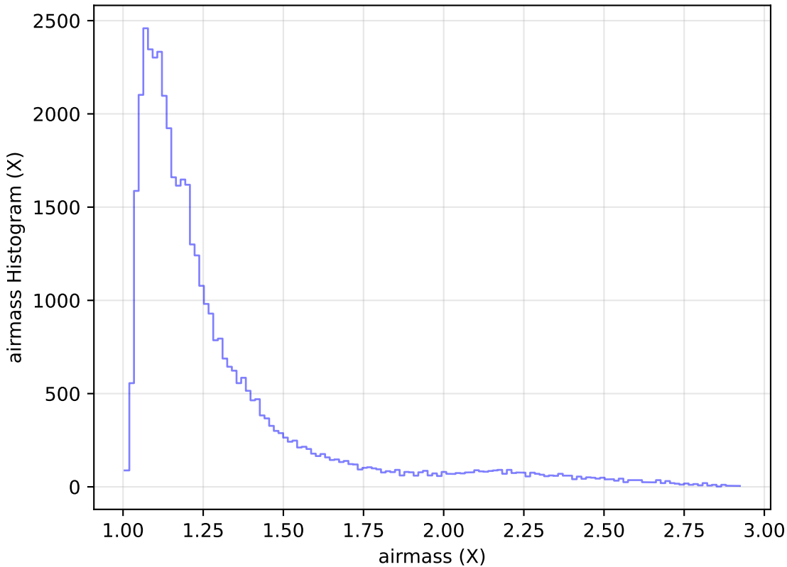
ddf_loaded_fl8_v3.4_10yrs Yr 1 z band: airmass Histogram
