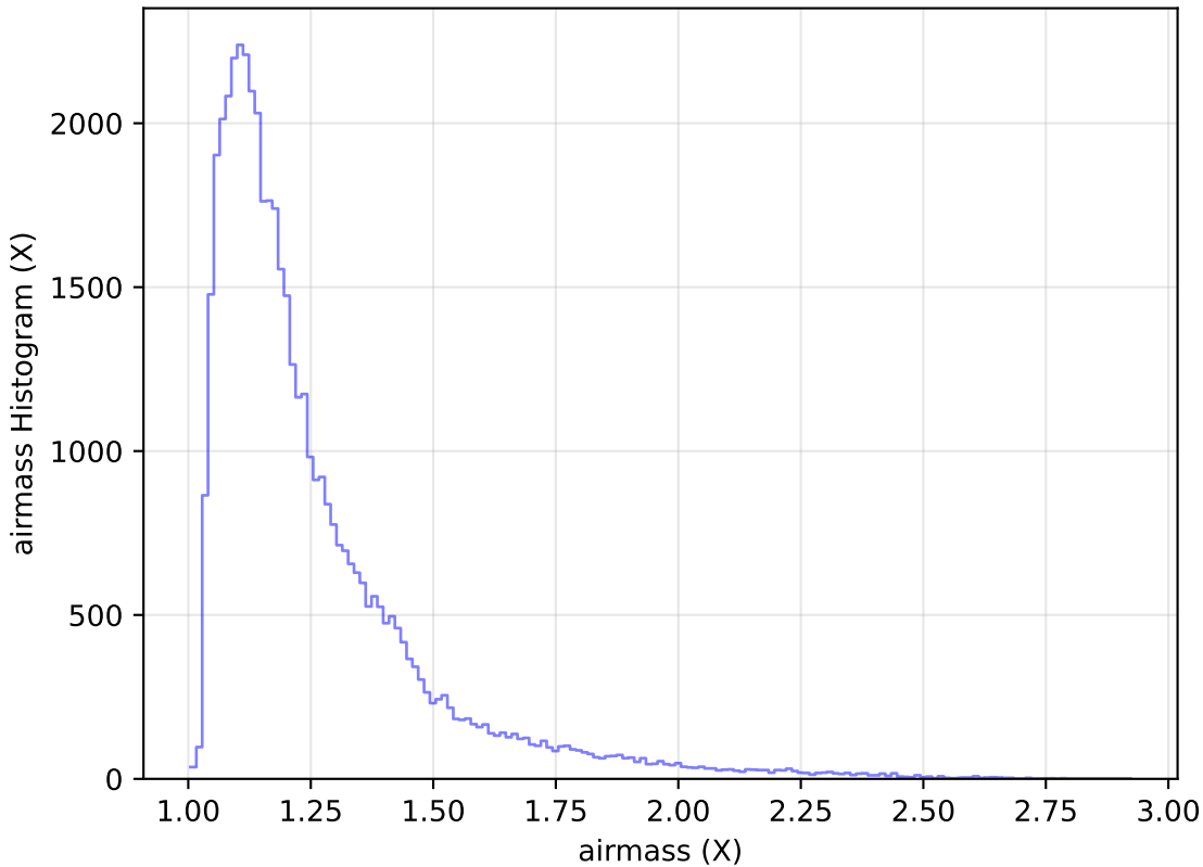
ddf_loaded_fl8_v3.4_10yrs Yr 1 y band: airmass Histogram
