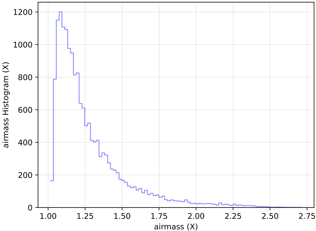
ddf_loaded_fl8_v3.4_10yrs Yr 1 u band: airmass Histogram
