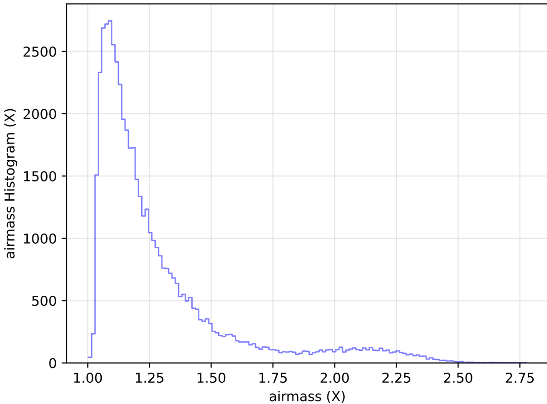
ddf_loaded_fl8_v3.4_10yrs Yr 1 r band: airmass Histogram
